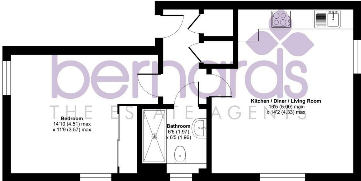
FIRST FLOOR
